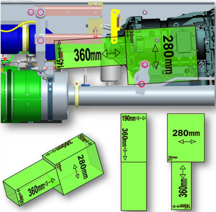
Figure 3-15 K270 PTO Clearances
