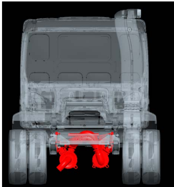
Figure 4-5.3: Back view of Horizontal Crossover DPF and SCR with Horizontal Tailpipe
