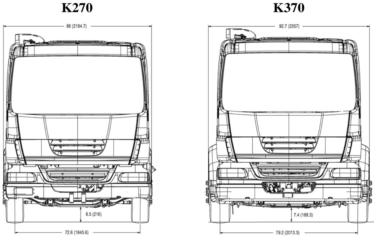
Figure 3-4. K270/K370 W/19.5 Tires Front View: Width and Ground Clearance Measurements: inches (mm).
